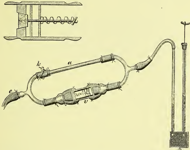
FIG. 36. THE MAXIMUM MANOMETER OF GOLTZ AND GAULE.
